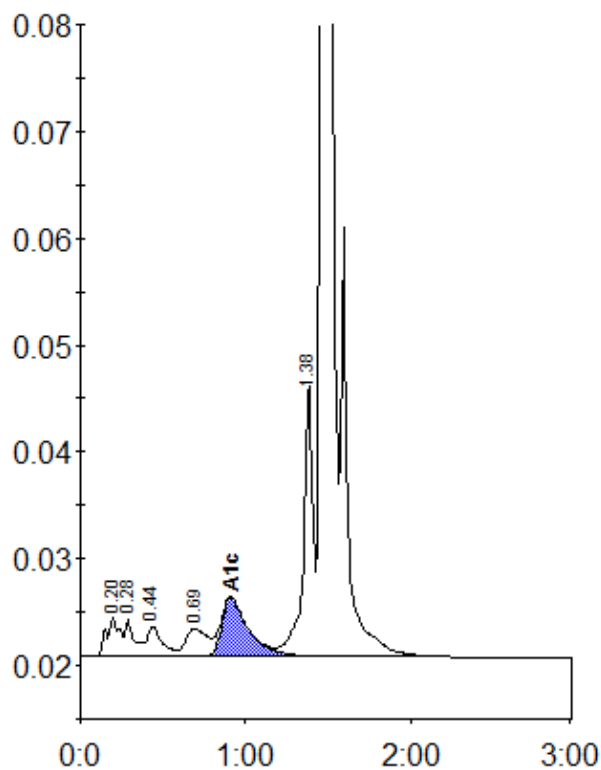
Peak table - ID: 10401233
